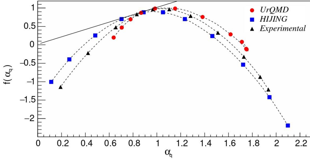
Fig. 5: shows the variation of f(\alpha_q) against f(\alpha_q) versus \alpha_q for 28Si-AgBr collisions at 14.5A GeV/c.
