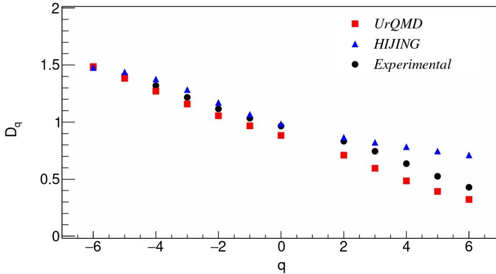
Fig. 4: Plot of D_q against q for 28Si-AgBr collisions at 14.5A GeV/c.
