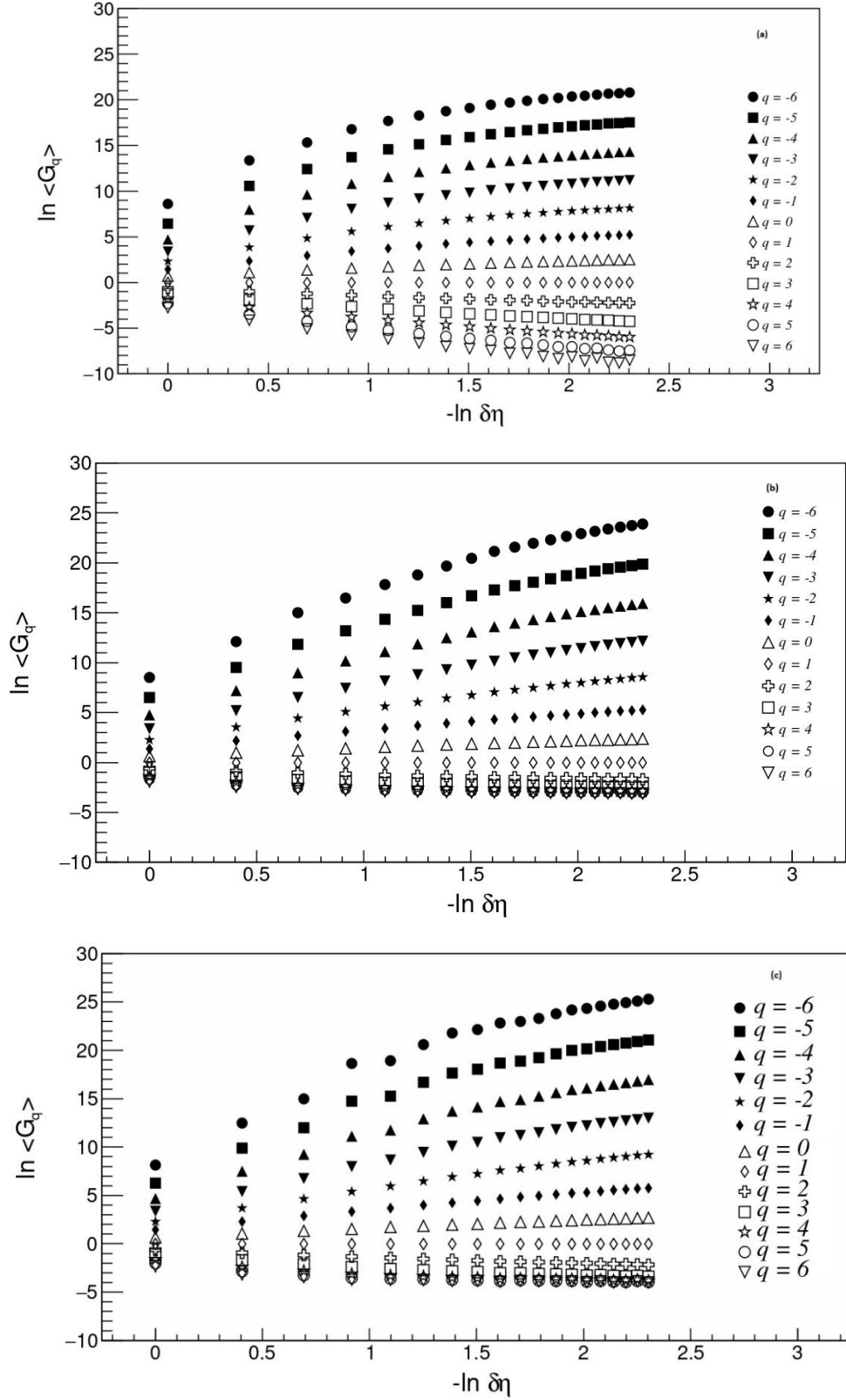
Fig. 2: Variations of \ln \langle G_q \rangle with -\ln \delta\eta for (a) UrQMD, (b) HIJING and (c) Experimental data.
