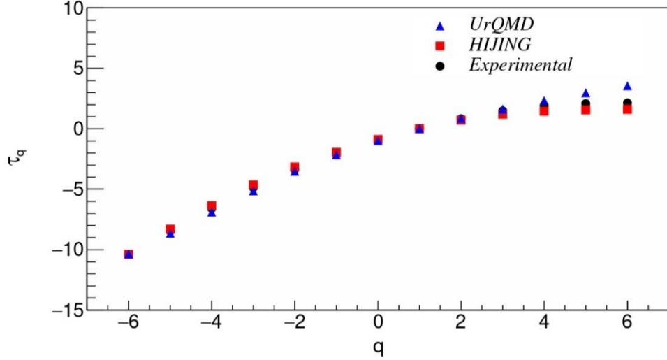
Fig. 3: Variation of \tau_q versus q for 28Si-AgBr collisions at 14.5A GeV/c.
