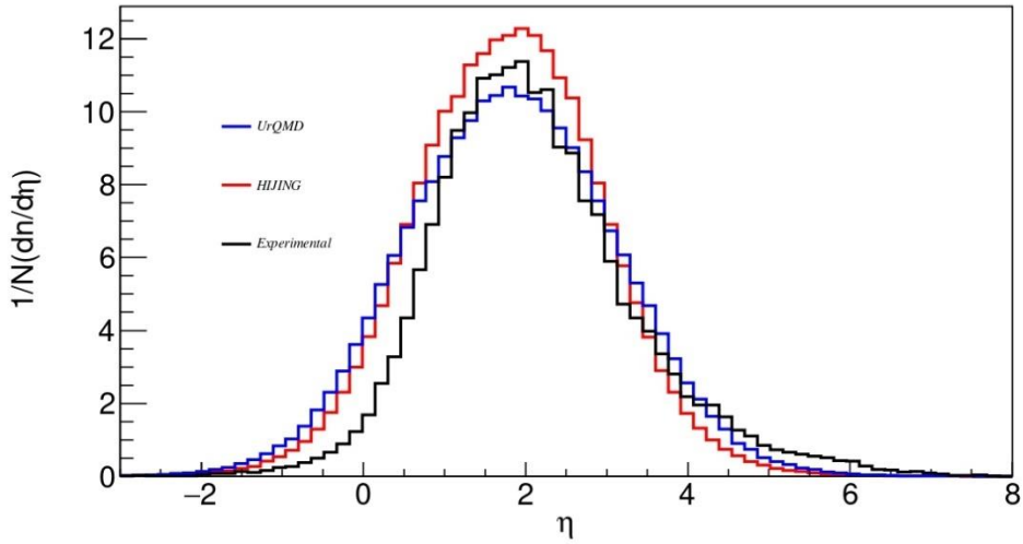
Fig. 1: Pseudorapidity distribution for UrQMD, HIJING, and Experimental data.
